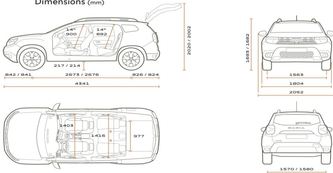
Dimensions (mm)
